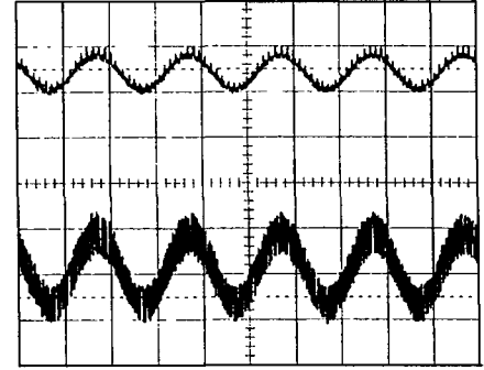
IC4051 pins 7/16 0v5 p.p. at 0.5m sec
