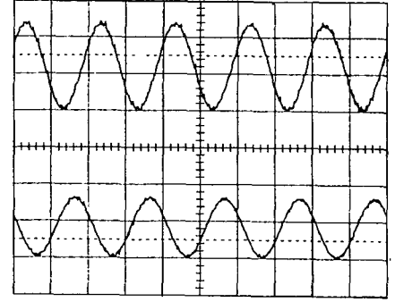
IC402 pins 10/23 0v8 p.p. at 0.5m sec
