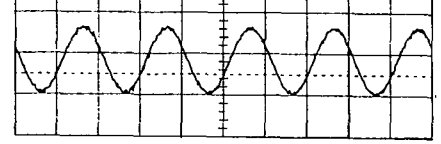
IC402 pins 10/23 0v8 p.p. at 0.5m sec
