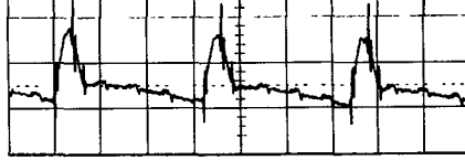
Q752 collector 0v52 p.p. at 20 \mu sec
