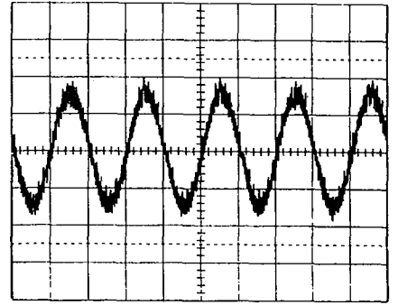
IC451 pins 7/8 0v76 p.p. at 0.5m sec
