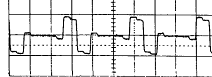
IC201 pin 29 0v9 p.p. at 20 \mu sec
