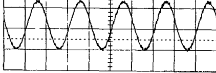
IC402 pins 7/26 1v2 p.p. at 0.5m sec
