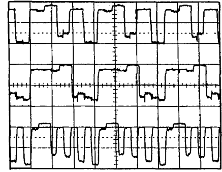
Q802 collector 90v p.p. at 20 \mu sec
