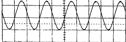
IC451 pins 11/12 1v2 p.p. at 0.5m sec
