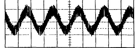
IC4051 pins 8/15 1v2 p.p. at 0.5m sec
