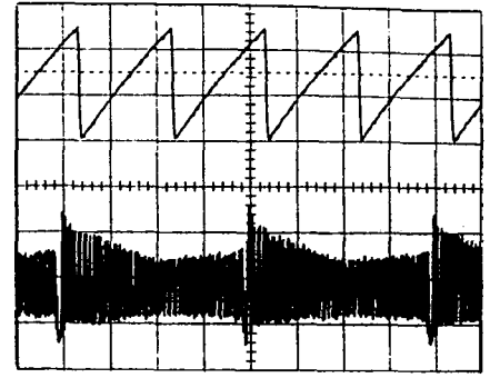
IC201 pin 42 1v25 p.p. at 10m sec
