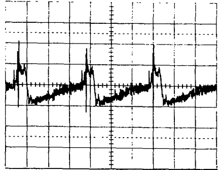
IC201 pin 16 170mV p.p. at 20 \mu sec
