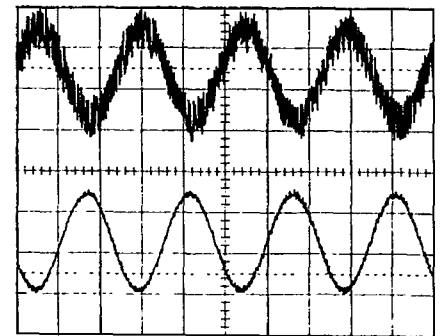
IC4450 pins 8/10 1v3 p.p. at 1m sec
