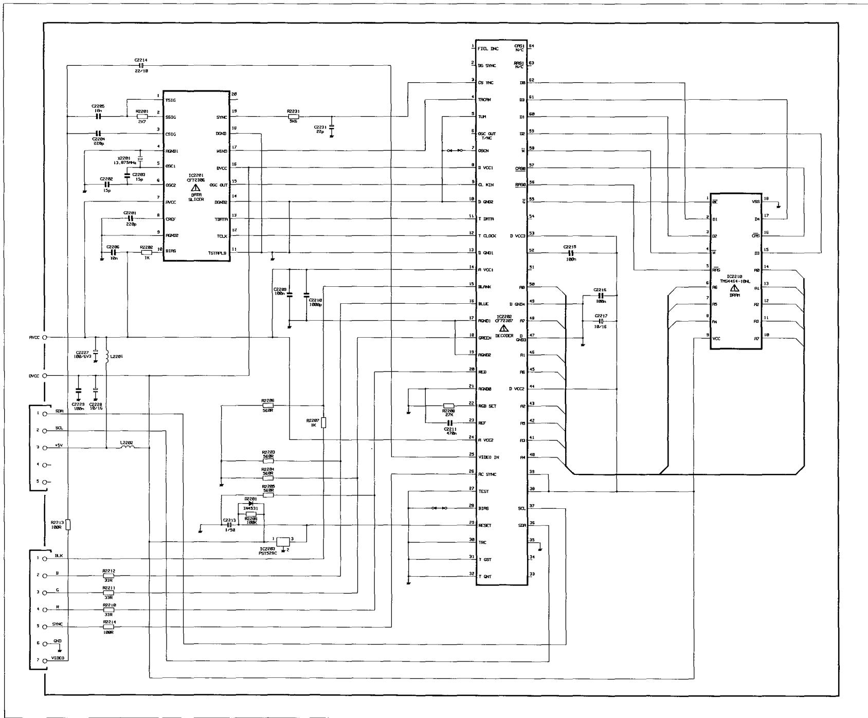
TELETEXT CIRCUIT VIDEOTEXT-PLATINE
