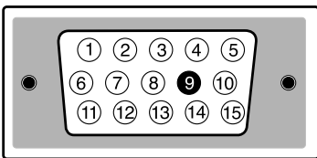
D-Sub miniature connector
