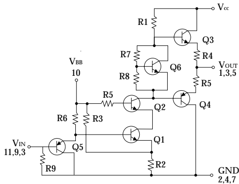
Simplified Schematic Diagram (One Channel)
