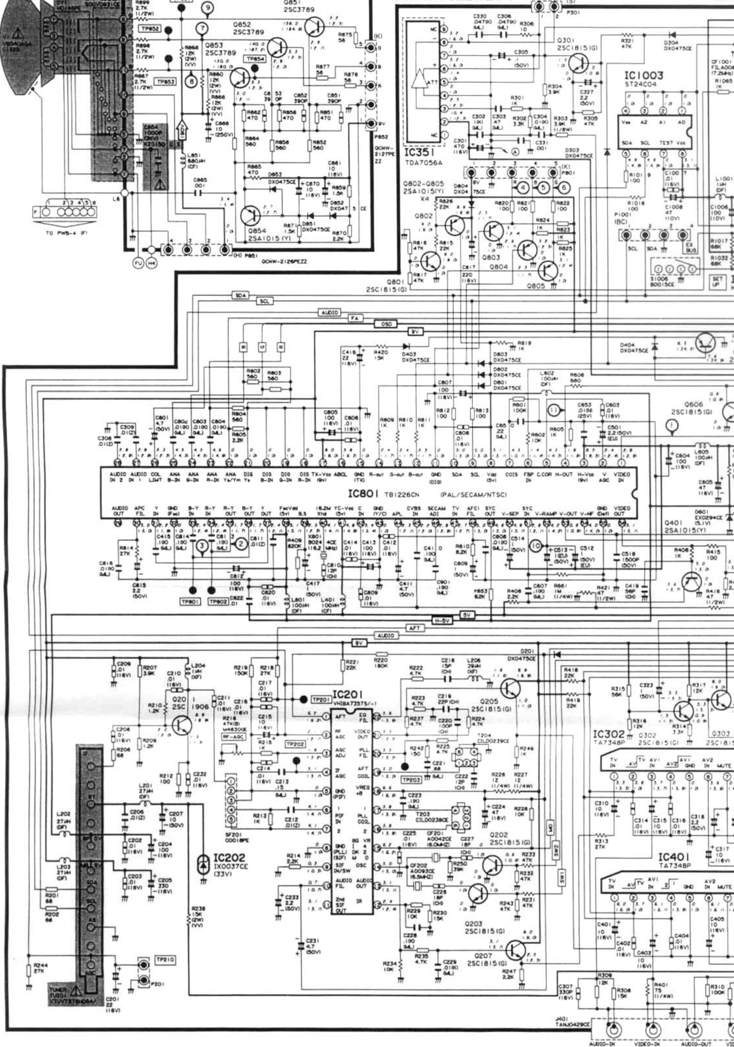
PWB-A (MAIN UNIT) DUNT9322WEV4
