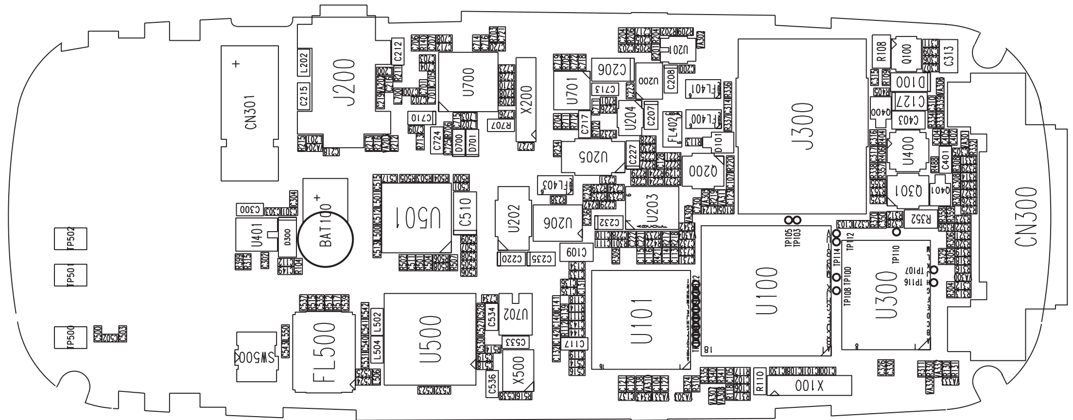
Figure 8-1 B2070 BOTTOM SIDE PCB LAYOUT
