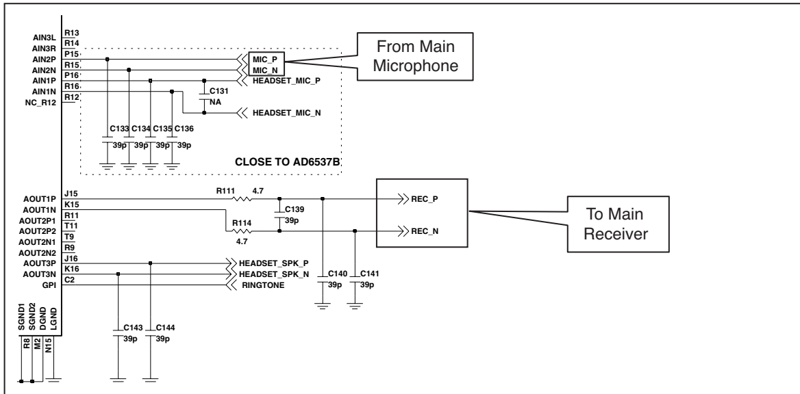
Figure 3-20 B2000 MAIN SPEAKER/MIC CIRCUIT (AD6537B)
