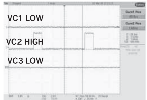
FEM Control DCS & PCS Graph 4-6(b)
