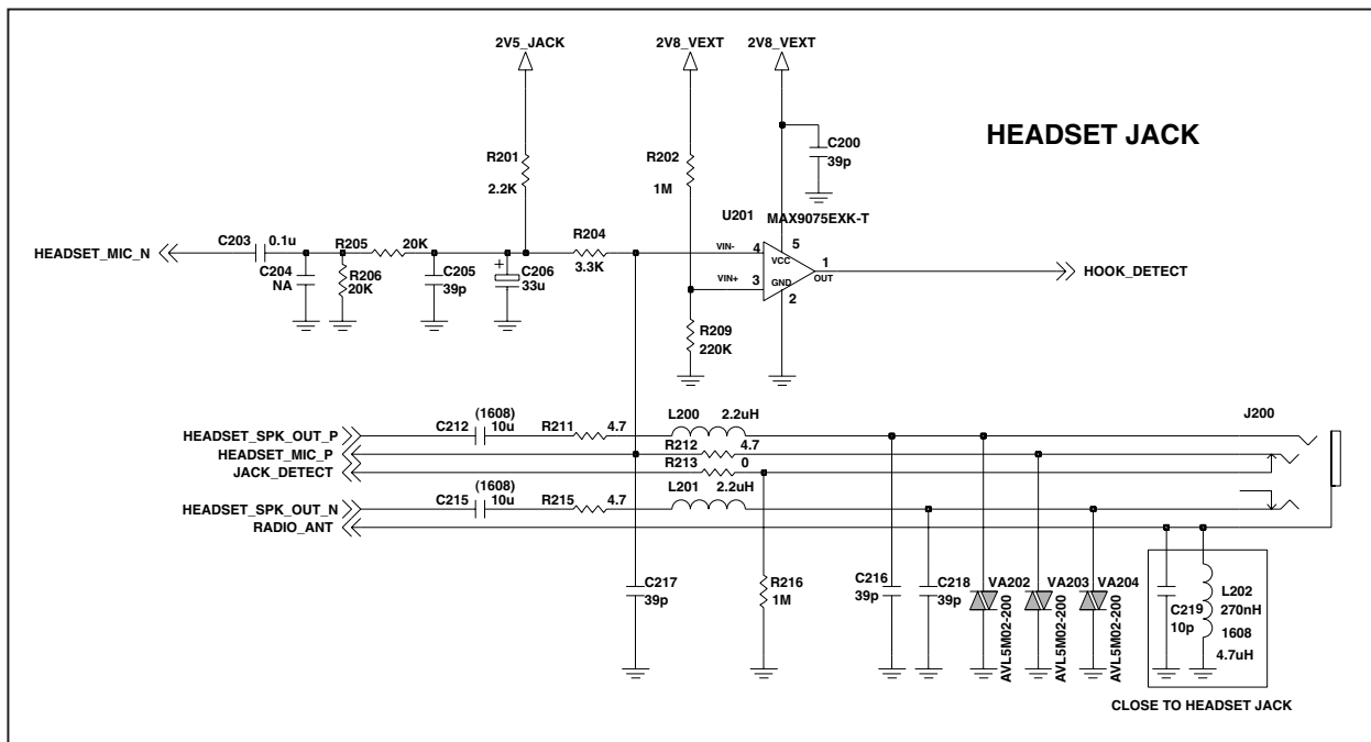
Figure 3-26 HEADSET JACK INTERFACE
