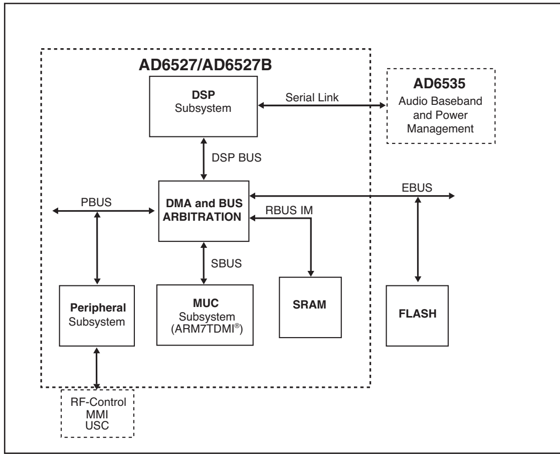
Figure 3-10 AD6527 ARCHITECTURE
