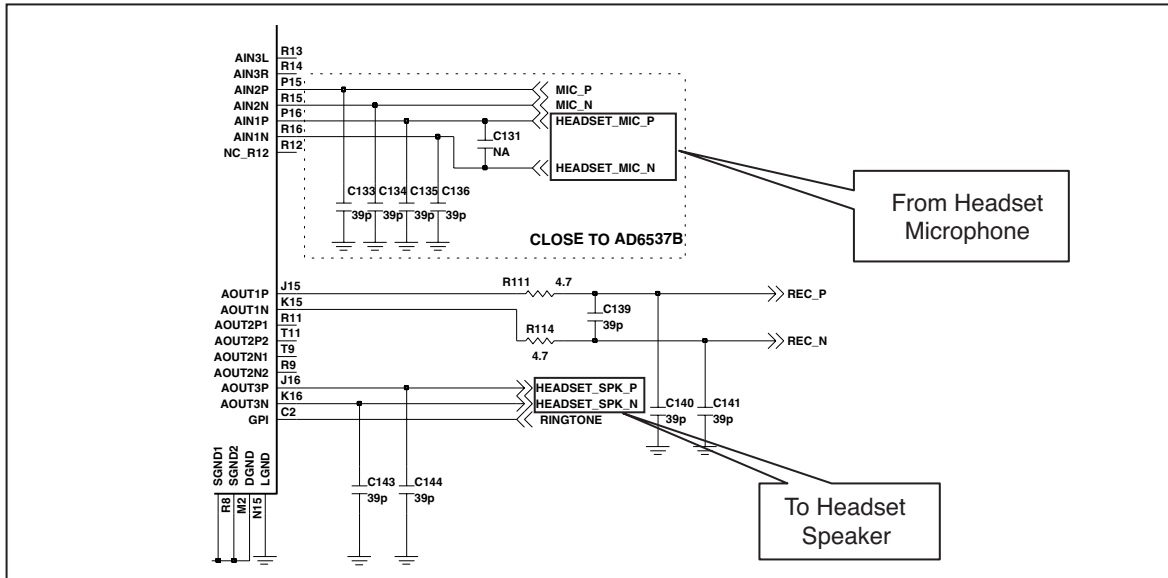
Figure 3-19 B2000 HEADSET SPEAKER/MIC CIRCUIT (AD6537B)
