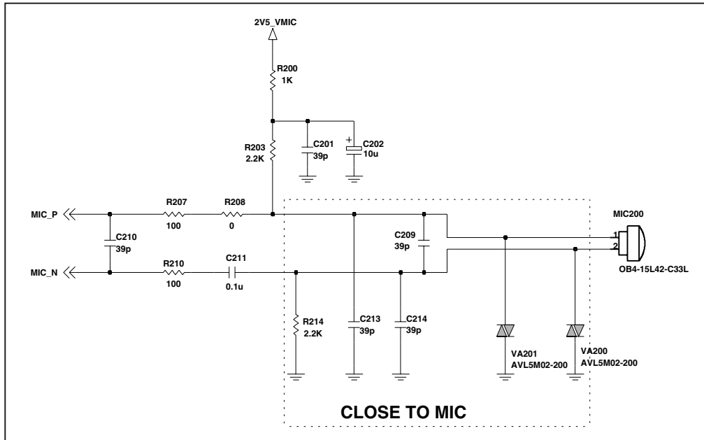
Figure 3-25 Connection between Microphone and AD6537B
