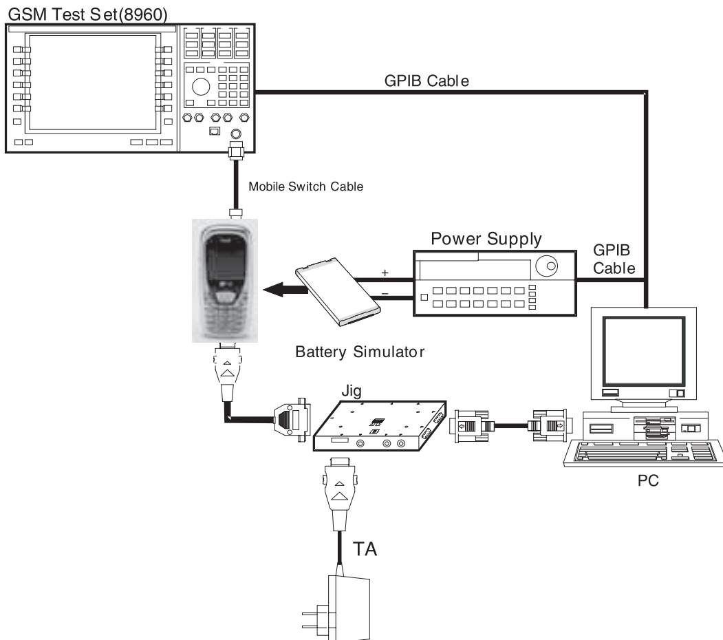
Figure 5-2 EQUIPMENT SETUP
