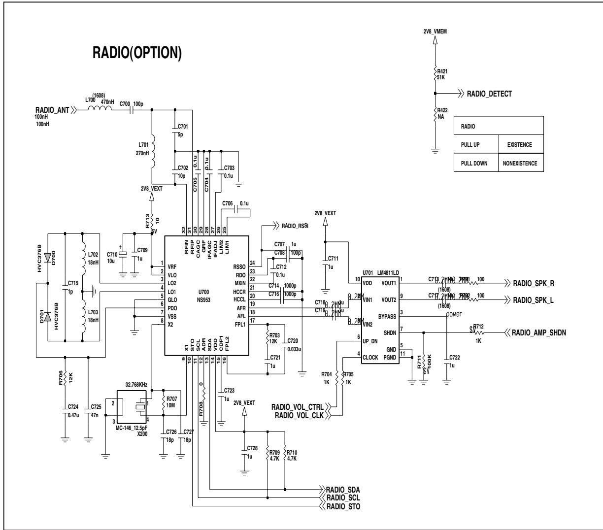
Figure 3-23 Radio Circuit
