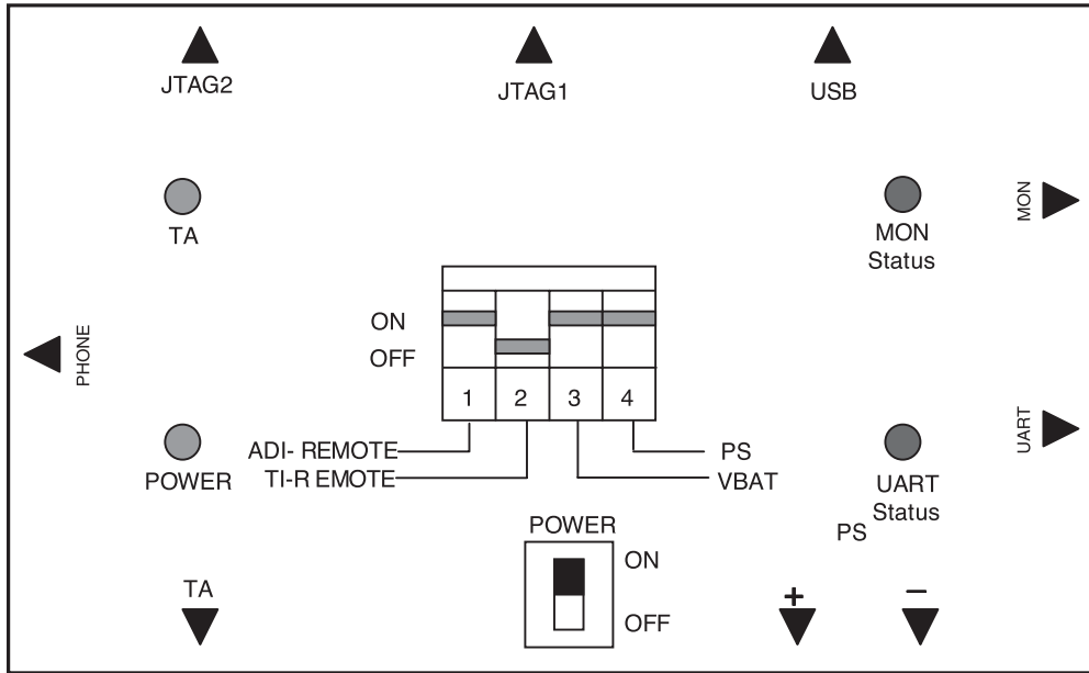
Figure 5-3 THE TOP VIEW OF TEST JIG
