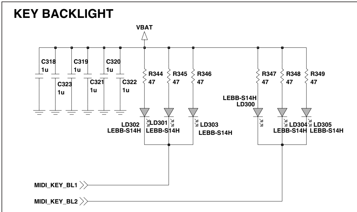
Figure 3-27 KEY BACK-LIGHT ILLUMINTION
