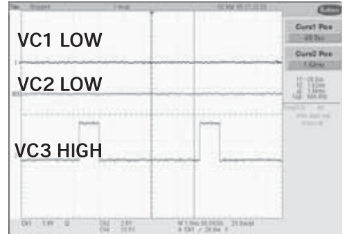
FEM Control EGSM Graph 4-6(a)
