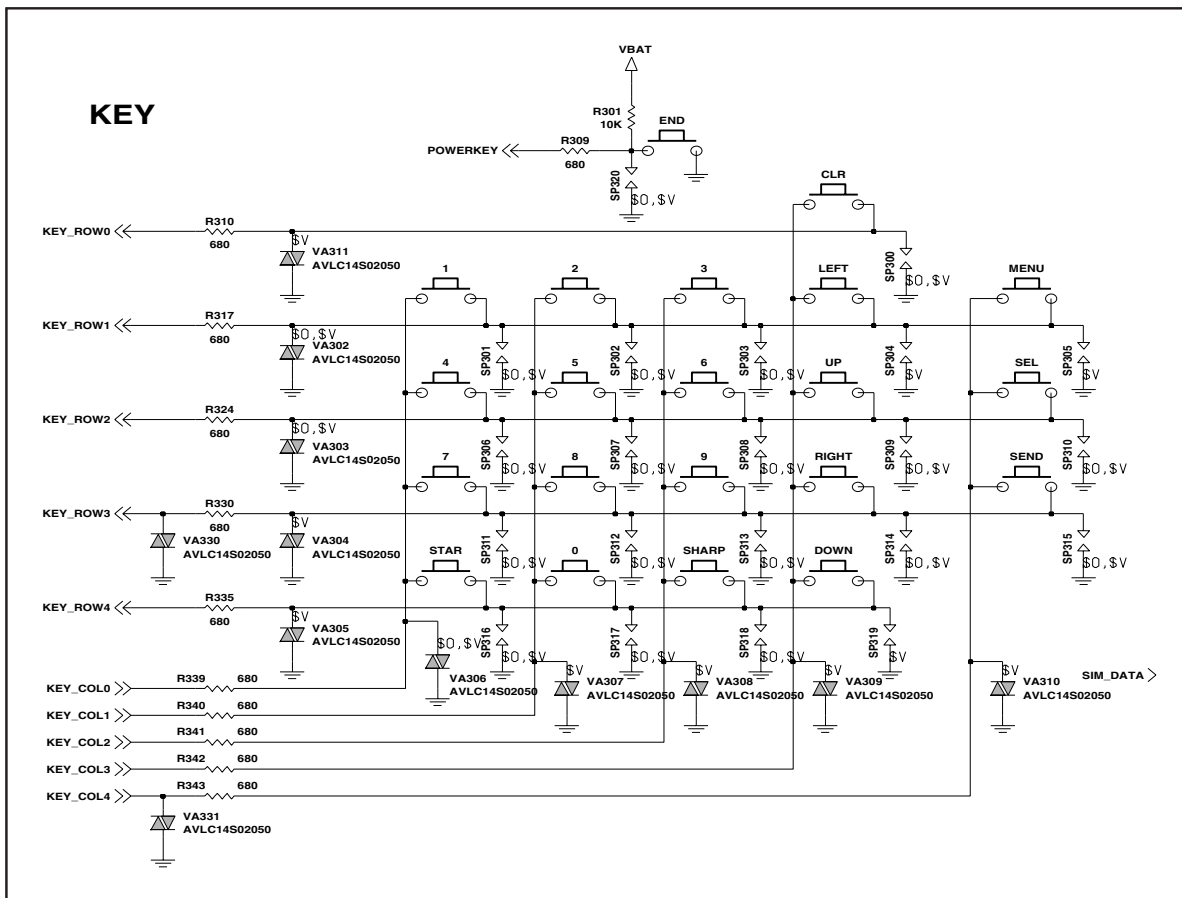
Figure 3-24 Keypad Switches and Scanning
