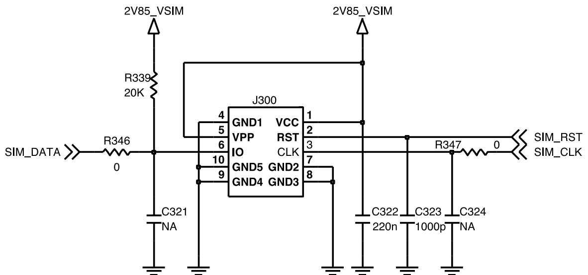
SIM CONNECTOR
