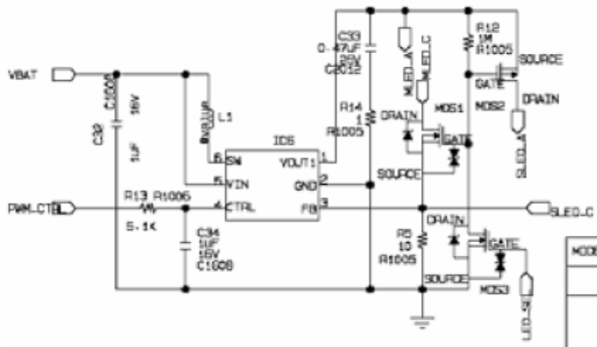
Figure. Charge Pump Circuit for Main LCD Backlight
