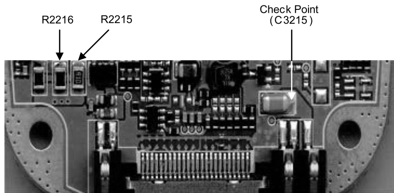
Figure 4-5. Power Source Block ⑤
